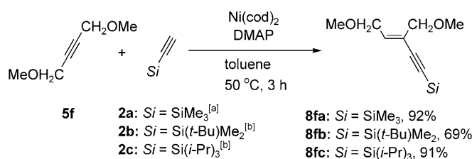
Scheme 1. Reaction of 1,4-dimethoxy-2-butyne ( 5f ) with silylacetylenes 2a–c . Reaction conditions: [a] [Ni(cod) 2 ]:[Ligand]:[ 5f ]:[ 2 ] = 0.025:0.15:0.5:1.5 (in mmol). [b] [Ni(cod) 2 ]:[Ligand]:[ 5f ]:[ 2 ] = 0.075:0.0125:0.25:0.75 (in mmol).
