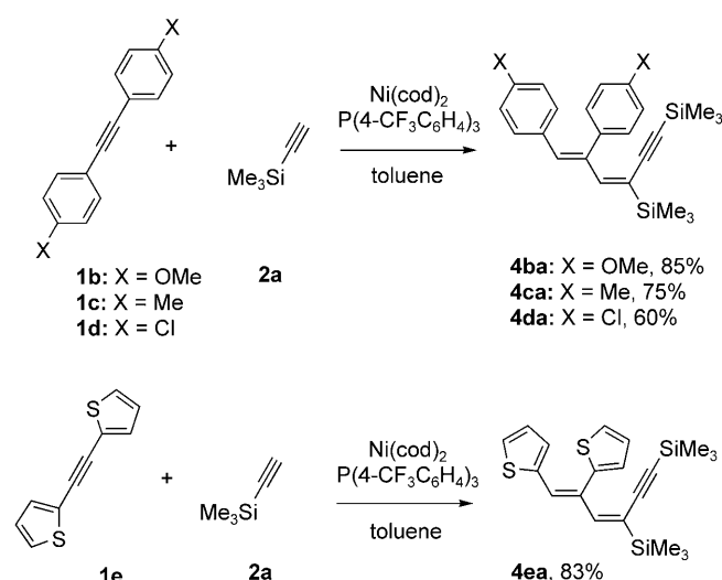
Scheme 2. Reaction of diarylacetylenes 1b–e with silylacetylene 2a to give dienyne 4 . Reaction conditions: [Ni(cod) 2 ]:[P(4-CF 3 C 6 H 4 ) 3 ]:[ 1 ]:[ 2a ] = 0.00625:0.00625:0.25:0.75 (in mmol).
